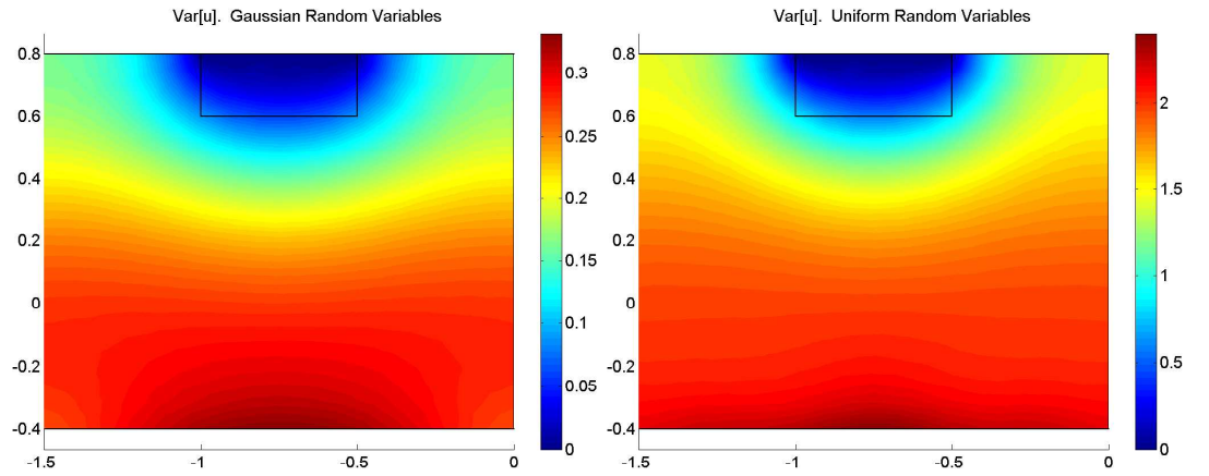
Figure 4: Results for the computation of the variance of the solution, Var[u] .
