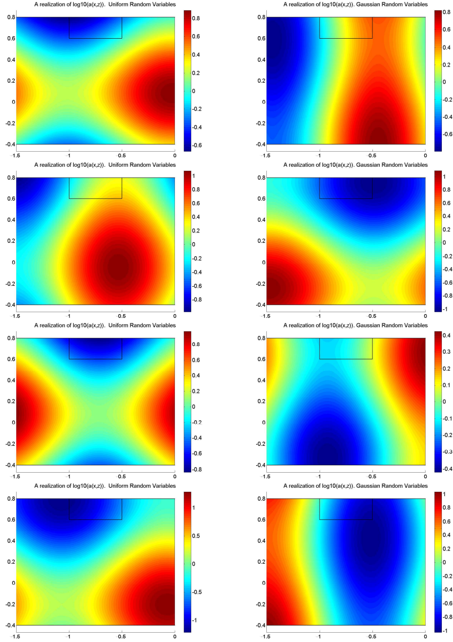
Figure 2: Some realizations of \log(a) .
