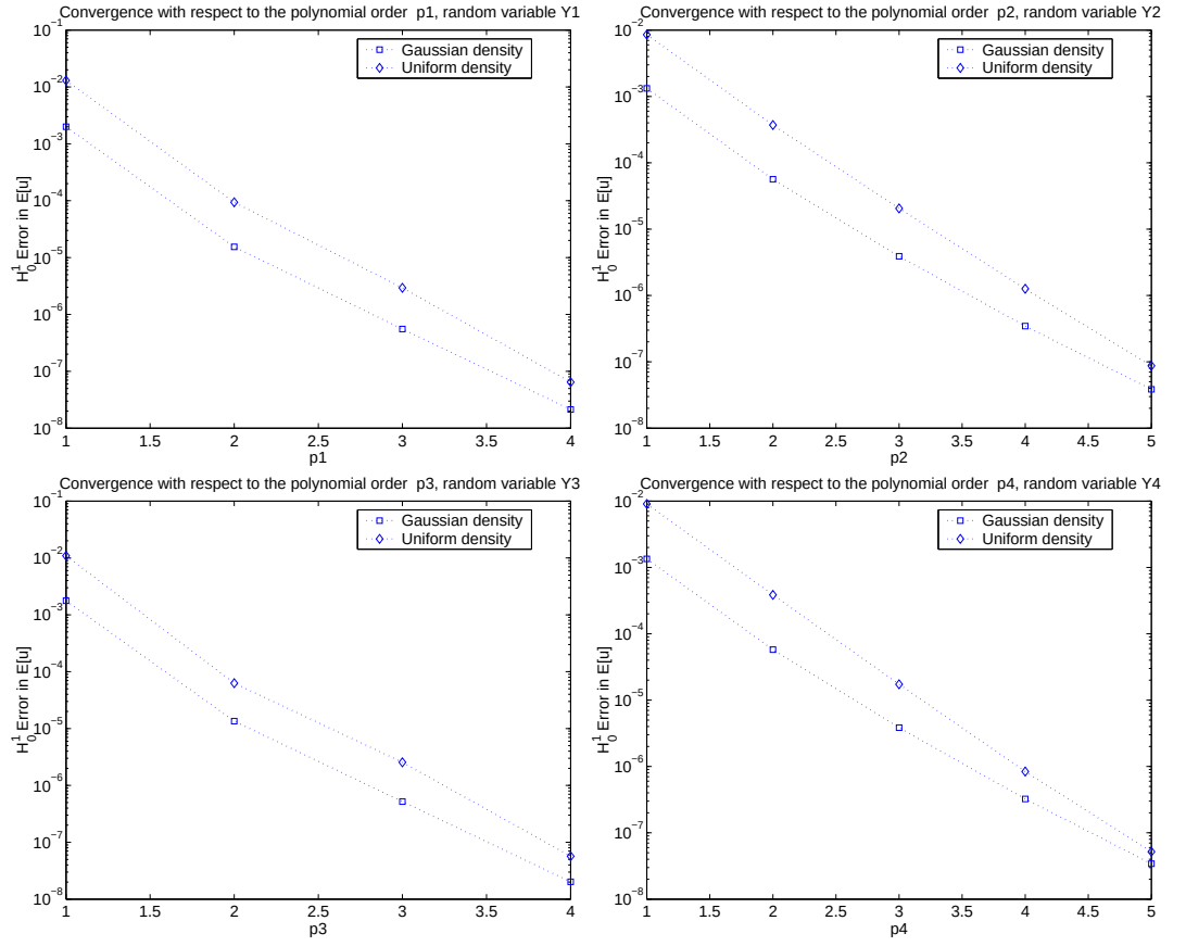
Figure 6: Convergence results for the approximation of the expected value, E[u] .
