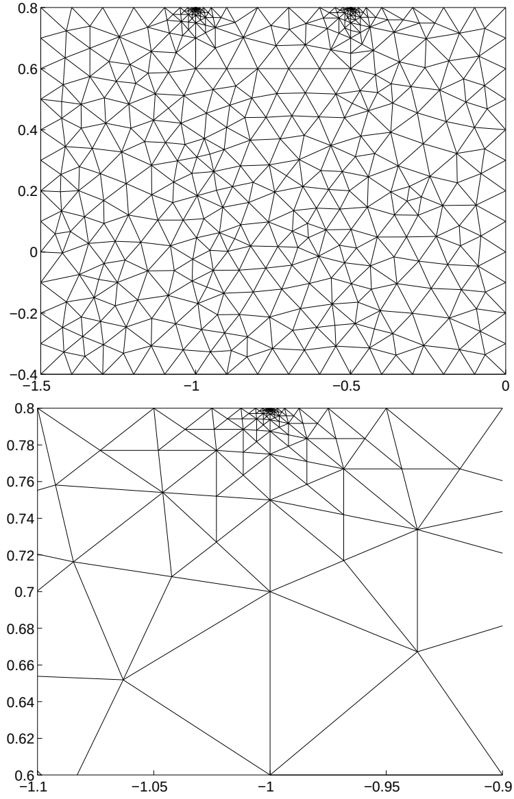
Figure 5: Top: Unstructured grid for the spatial discretization. The corresponding finite element spaces are the span of continuous functions that are piecewise polynomials with degree five. Bottom: Detail of the mesh refinement near the left singularity.
