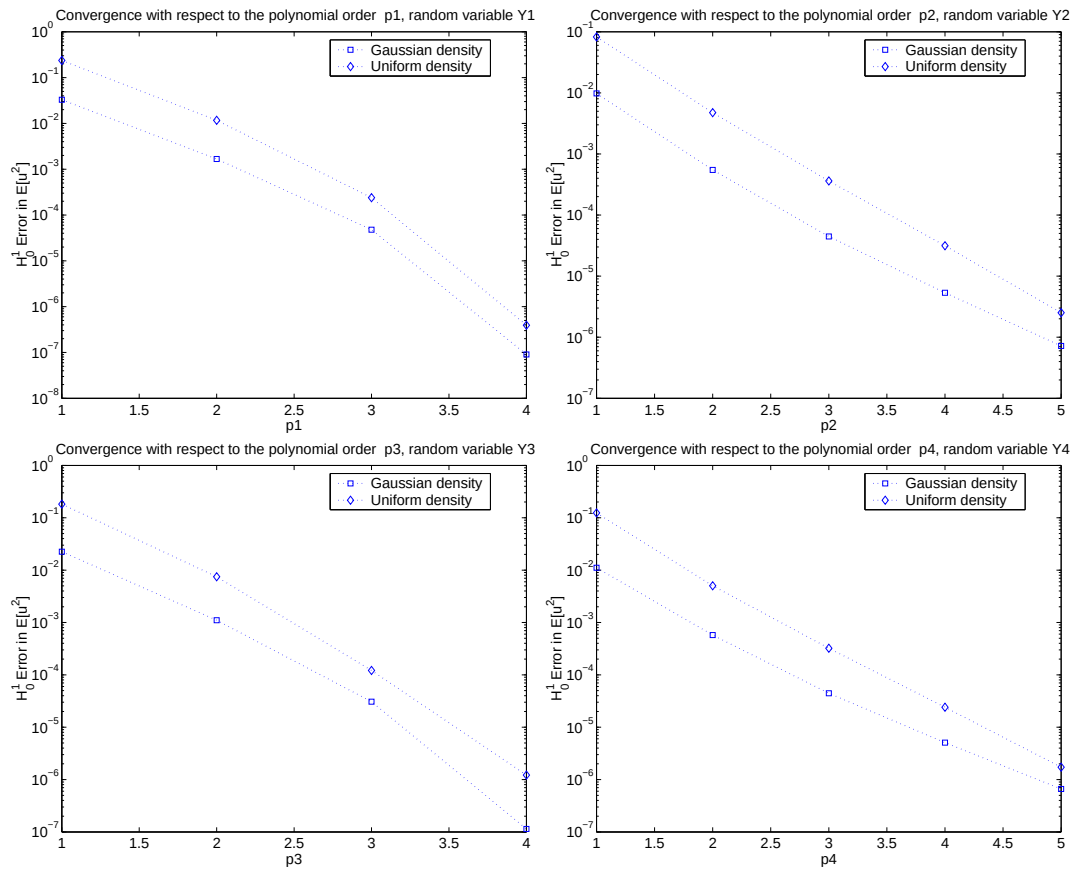
Figure 7: Convergence results for the approximation of the second moment, E[u^2] .
