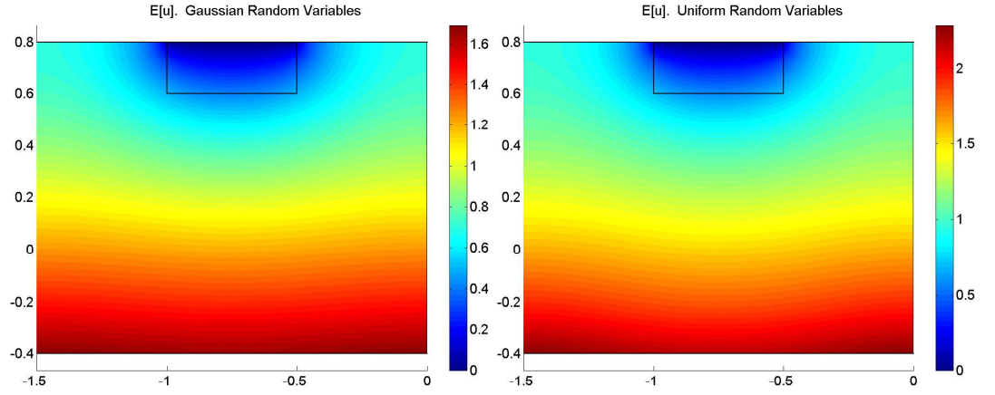
Figure 3: Results for the computation of the expected value for the solution, E[u] .
