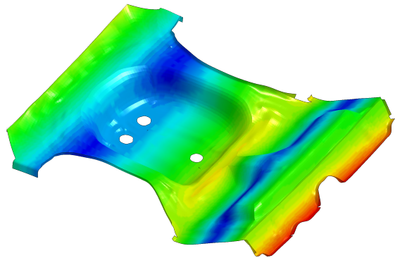
Figure 3: The seventh mode of a reconstructed rear car floorboard using bicubic NURBS patches is shown.
