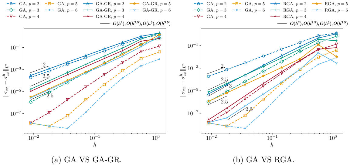
Figure 18: Infinite plate with a hole: Convergence rates of the L^2 -norm error with respect to the stress component \sigma_{xx} , for various quadratures, degrees p = 2 to 6, and non-uniform meshes.
