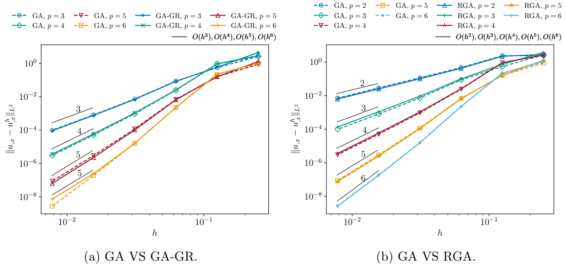
Figure 13: Biharmonic equation \Delta^2 u = f , where u(x, y) = \sin^2(2\pi x) \sin^2(2\pi y) : Convergence rates of the L^2 -norm error of the x -derivative of the solution u , for quadratures GA, GA-GR and RGA, and various basis degrees.
