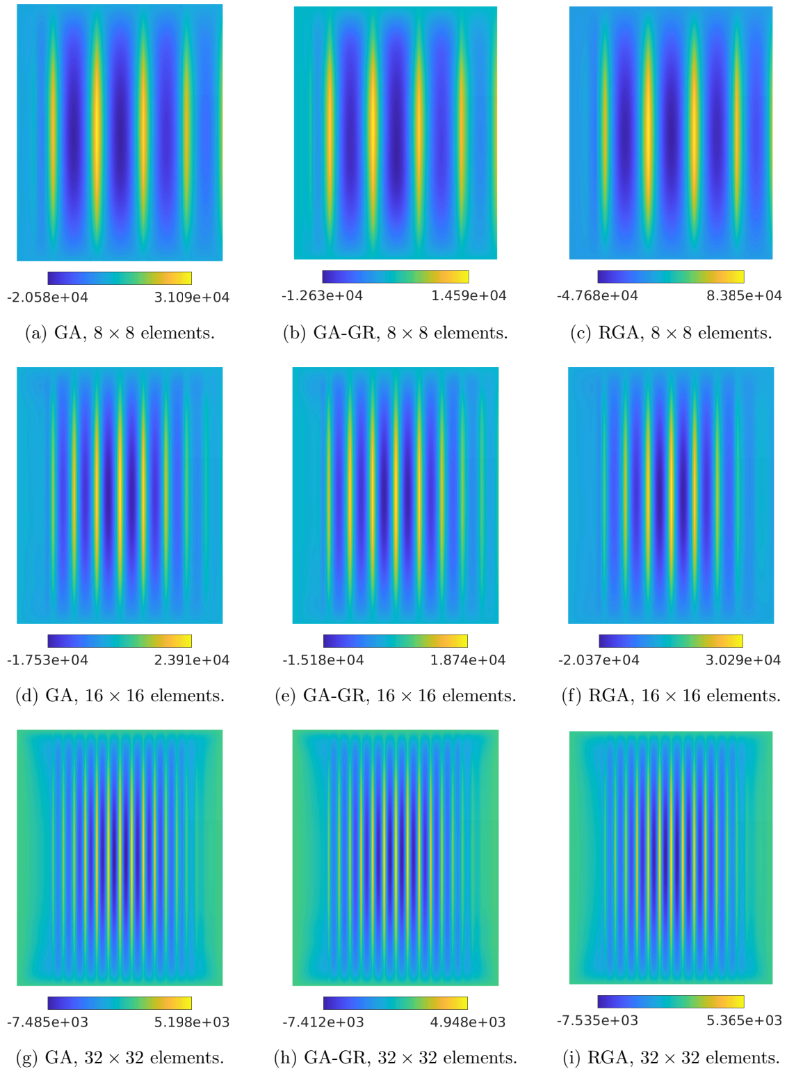
Figure 34: Scordelis-Lo roof modeled as an RM shell: Membrane force n_{11} for GA (left), GA-GR (middle) and RGA (right), degree p = 2 , and various numbers of elements.
