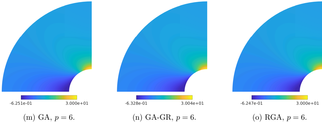
Figure 19: Infinite plate with a hole: Stress \sigma_{xx} for quadrature rules GA (left), GA-GR (middle) and RGA (right), degrees p = 2 to 6, 12 \times 12 elements, non-uniform meshes. Note that the stress concentration of a factor of 3 in \sigma_{xx} is accurately captured in all cases.
