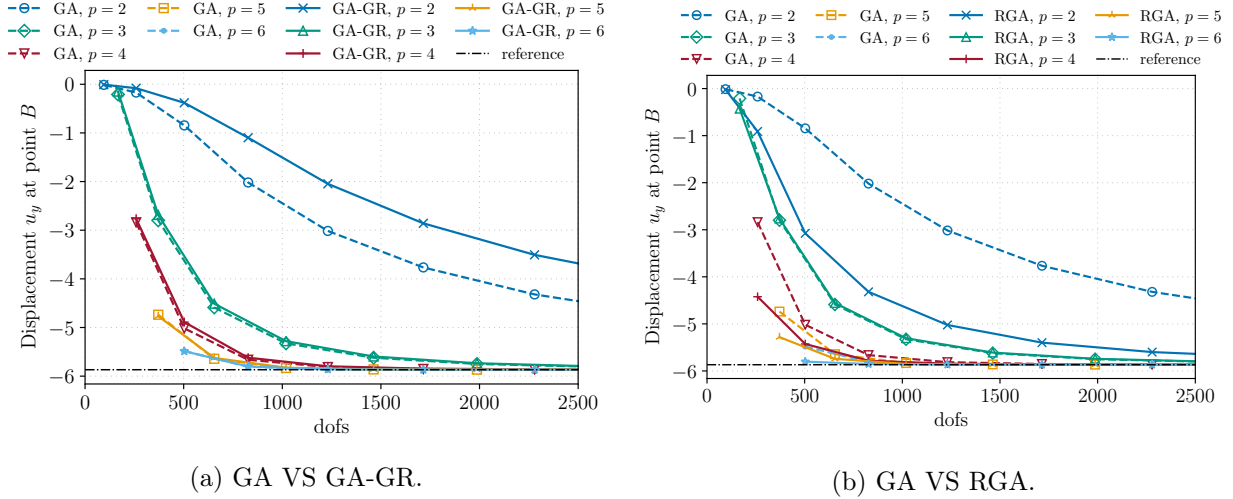
Figure 37: Hemispherical shell modeled as an RMC shell: Convergence of the displacement u_y at point B for load P = 200 with GA, GA-GR and RGA, degrees p = 2 to 6 , maximally smooth elements and 10 load steps.
