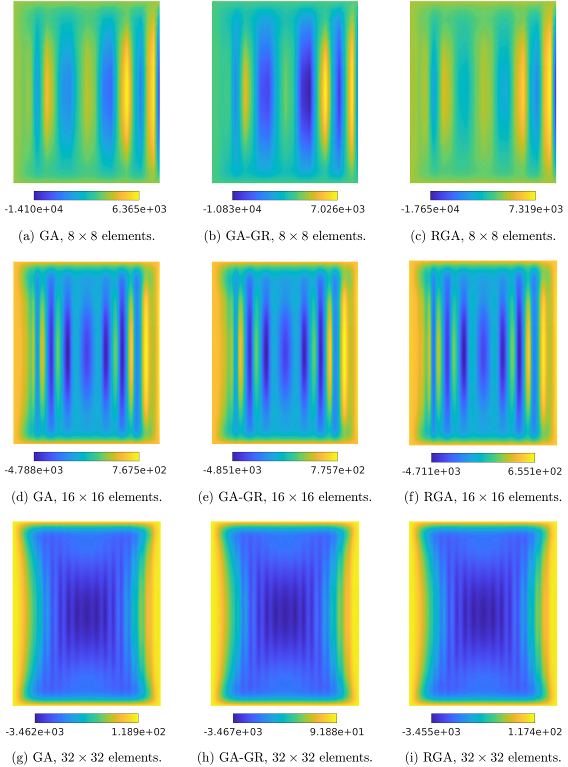
Figure 32: Scordelis-Lo roof modeled as a KL shell: Membrane force n_{11} for GA (left), GA-GR (middle) and RGA (right), degree p = 3 , and various numbers of elements.
