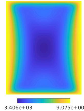
Figure 31: Scordelis-Lo roof modeled as a KL shell: Numerical reference of the membrane force n_{11} , calculated with full Gauss quadrature and 64 \times 64 maximally smooth elements, p = 6 .
