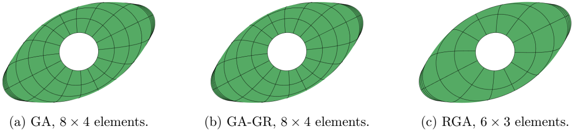
Figure 38: Hemispherical shell and the RMC shell: Deformed configurations with GA, GA-GR and RGA, maximally smooth quintic B-spline elements, P = 200 and 10 load steps, |u_y - u_{\text{ref}}|/|u_{\text{ref}}| < 5\% at point B .
