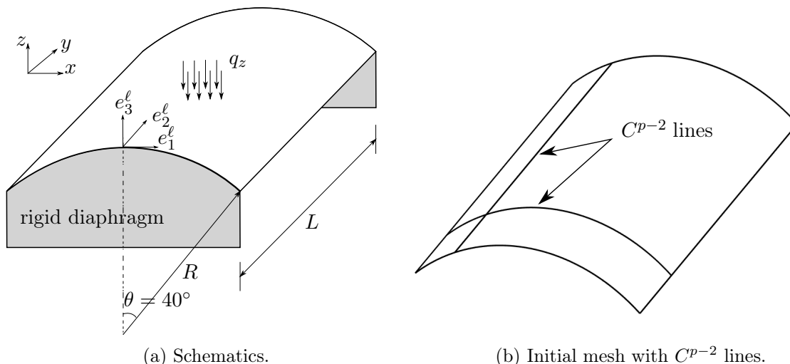
Figure 28: Schematic and initial mesh for the Scordelis-Lo roof problem.
