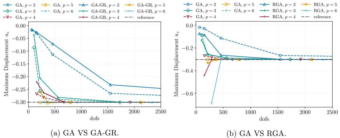
Figure 30: Scordelis-Lo roof modeled as an RM shell: Convergence of the maximum displacement u_z for GA, GA-GR and RGA, and degrees p = 2 to 6. The entire roof is modeled with an initial 2 \times 2 mesh as shown in Figure 28b.
