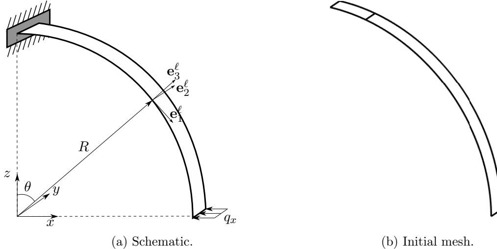
Figure 20: Cylindrical shell subject to transverse loading in the radial direction. \{e_i^\ell\}_{i=1}^3 is a local Cartesian coordinate basis used for calculating resultant forces [1].
