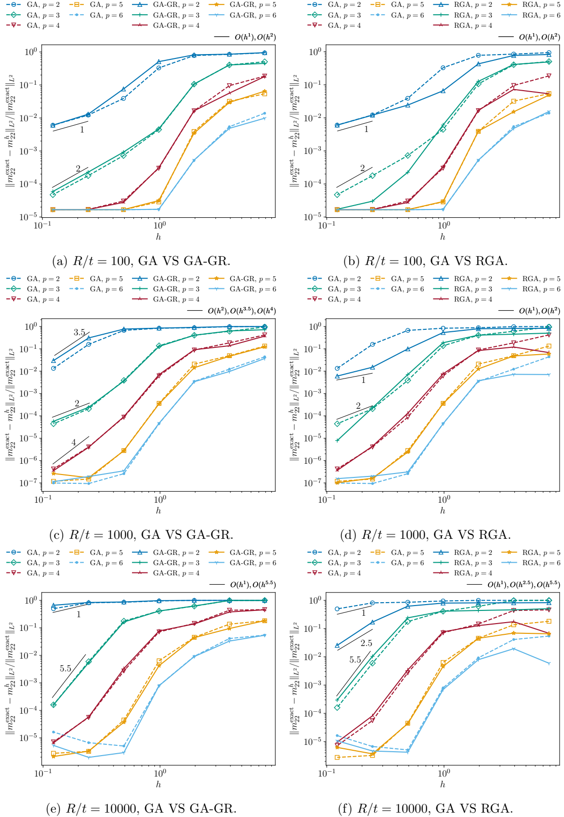
Figure 22: Cylindrical KL shell: Bending moment convergence rates for GA, GA-GR and RGA, increasing slenderness R/t = 100, 1000, 10000 , degrees p = 2 to 6 , and maximally smooth elements.
