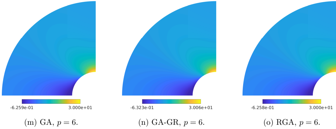
Figure 17: Infinite plate with a hole: Stress \sigma_{xx} for quadrature rules GA (left), GA-GR (middle) and RGA (right), degrees p = 2 to 6, 10 \times 10 elements, uniform meshes. Note that the stress concentration of a factor of 3 in \sigma_{xx} is accurately captured in all cases.
