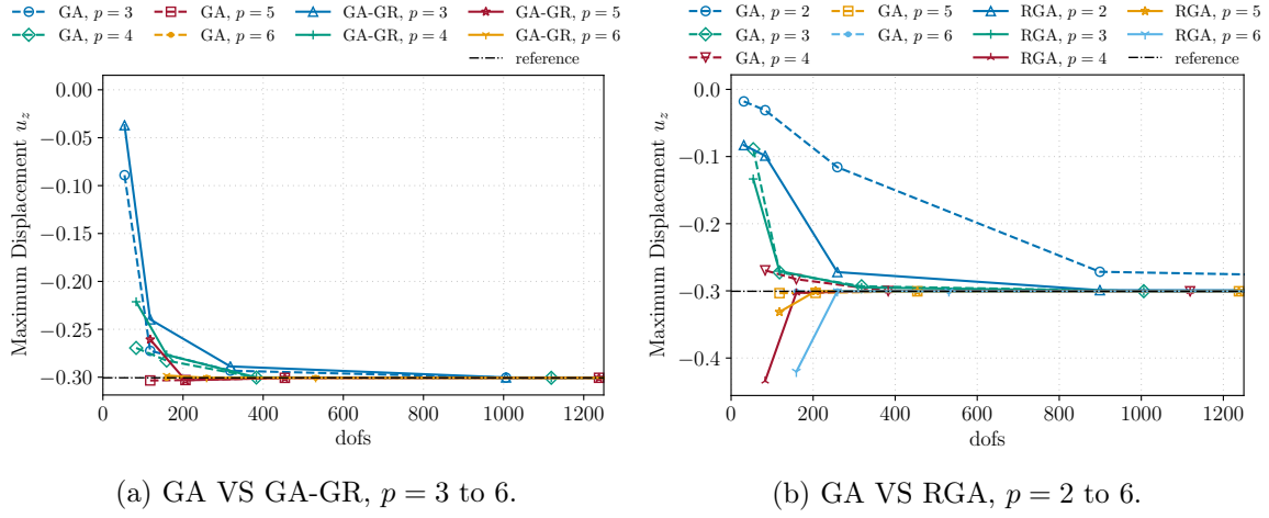
Figure 29: Scordelis-Lo roof modeled as a KL shell: Convergence of the maximum displacement u_z for GA, GA-GR and RGA, and various basis degrees. The entire roof is modeled with an initial 2 \times 2 mesh as shown in Figure 28b.
