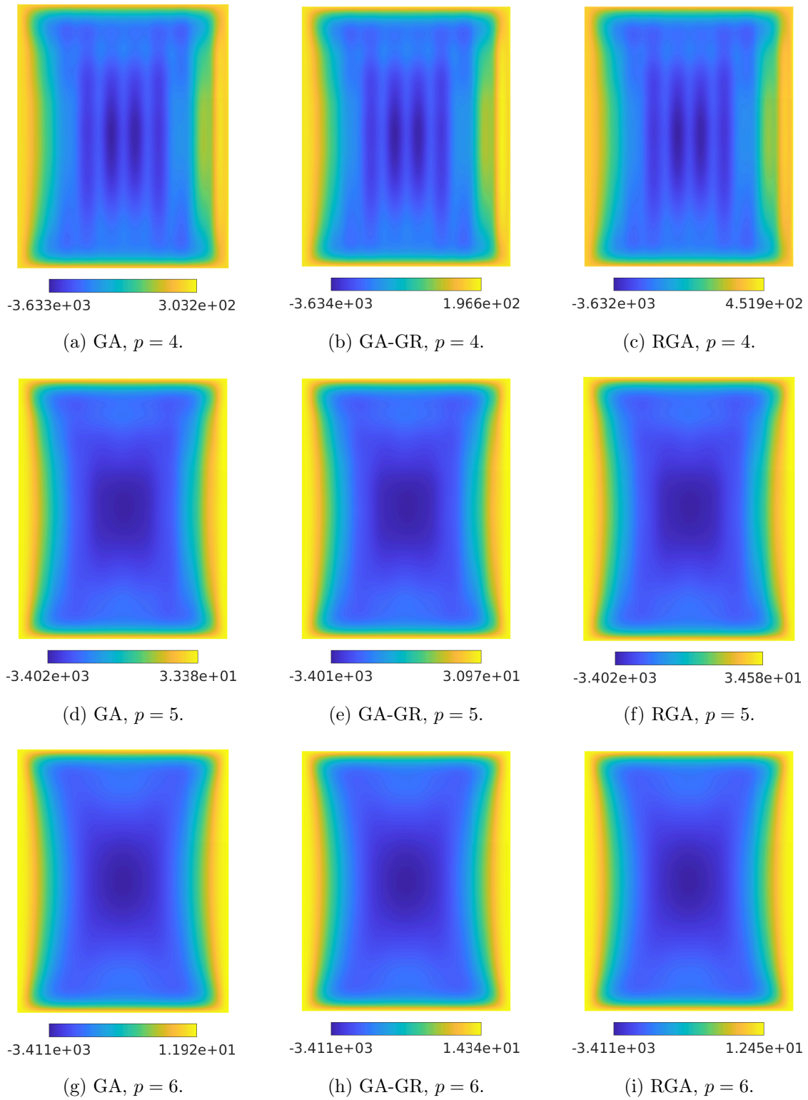
Figure 33: Scordelis-Lo roof modeled as a KL shell: Membrane force n_{11} for GA (left), GA-GR (middle) and RGA (right), degrees p = 4 to 6, and 16 \times 16 elements.
