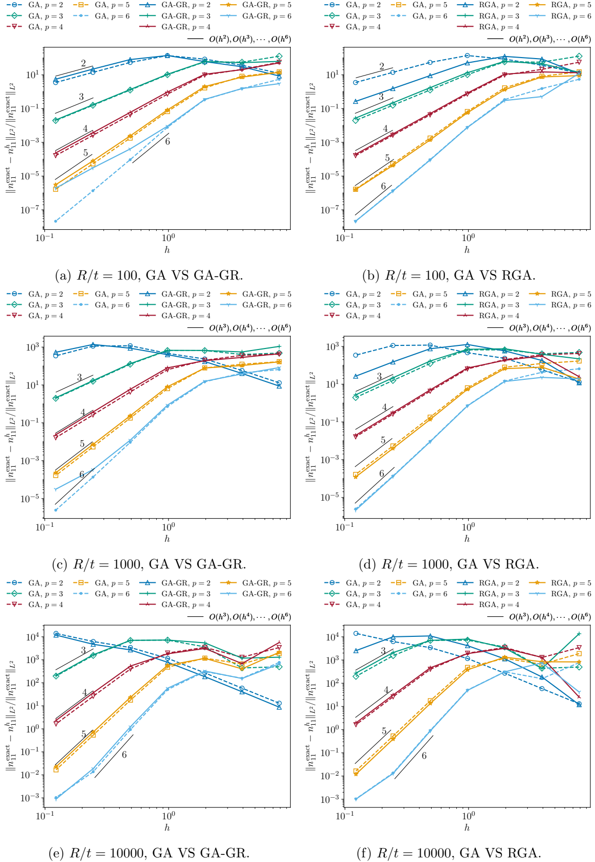
Figure 23: Cylindrical RM shell: Membrane force convergence rates for GA, GA-GR and RGA, increasing slenderness R/t = 100, 1000, 10000 , degrees p = 2 to 6, and maximally smooth elements.
