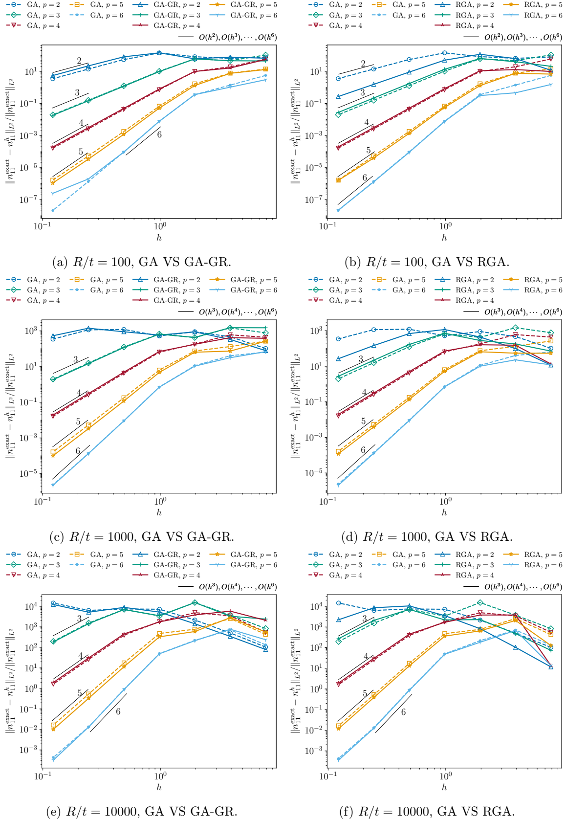
Figure 21: Cylindrical KL shell: Membrane force convergence rates for GA, GA-GR and RGA, increasing slenderness R/t = 100, 1000, 10000 , degrees p = 2 to 6 , and maximally smooth elements.
