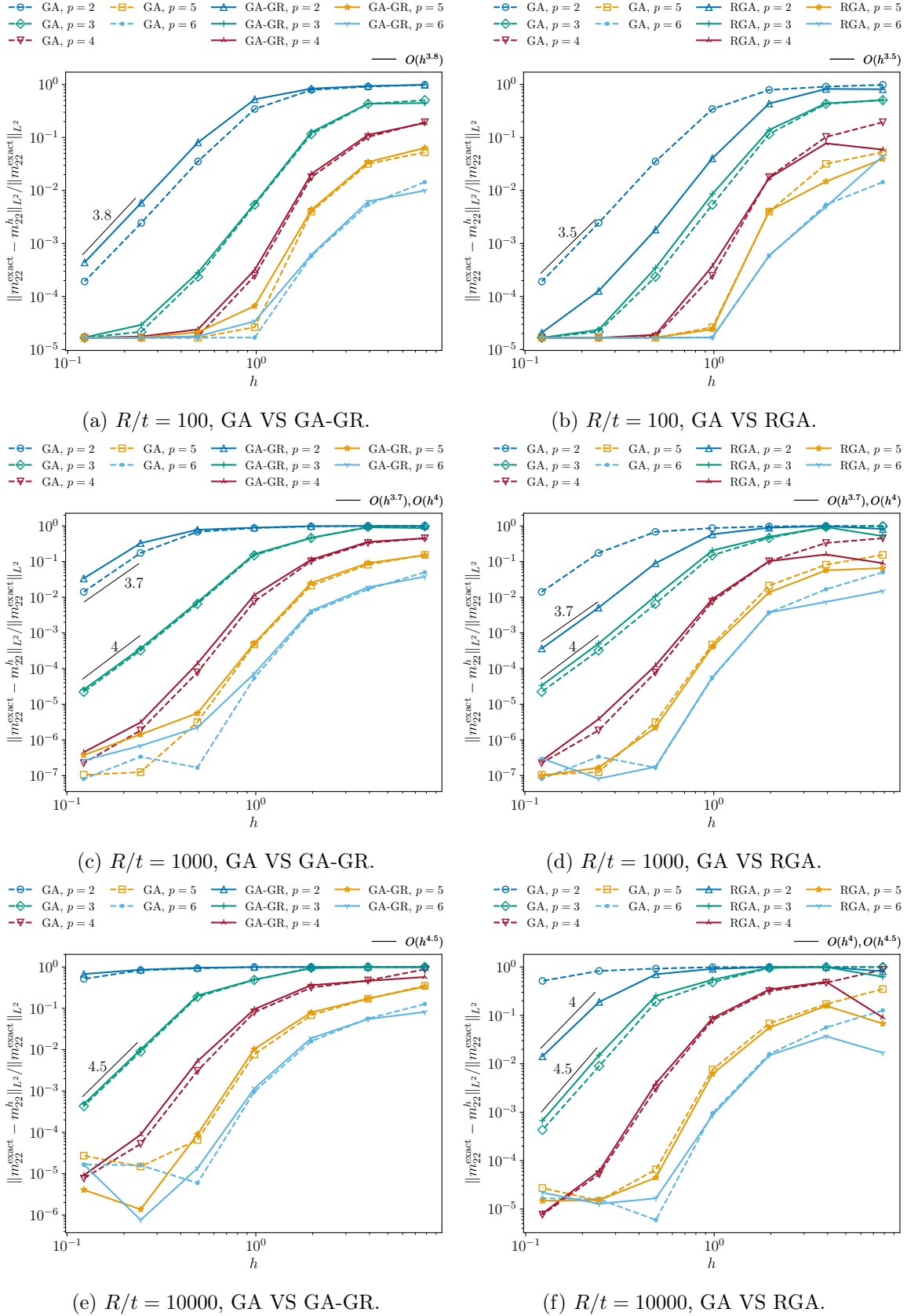
Figure 24: Cylindrical RM shell: Bending moment convergence rates for GA, GA-GR and RGA, increasing slenderness R/t = 100, 1000, 10000 , degrees p = 2 to 6, and maximally smooth elements.
